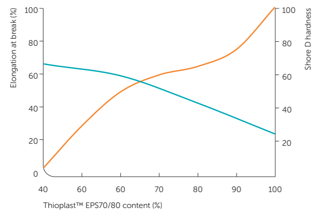
Figure 4: Increasing of elongation of cured Epoxy-resin by adding Thioplast™ EPS 70/80
