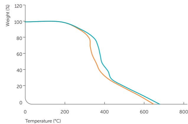
Figure 5: Thermogravimetric measurement of degradation of Thioplast™ EPS 70 / 80 and Bisphenol A/F resin
