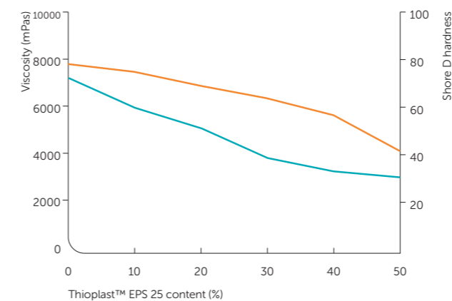
Figure 6: Relationship between viscosity and Thioplast™ EPS 25 content in Bisphenol A/F resins and Thioplast™ EPS 70 / EPS 80 at 25°C.
